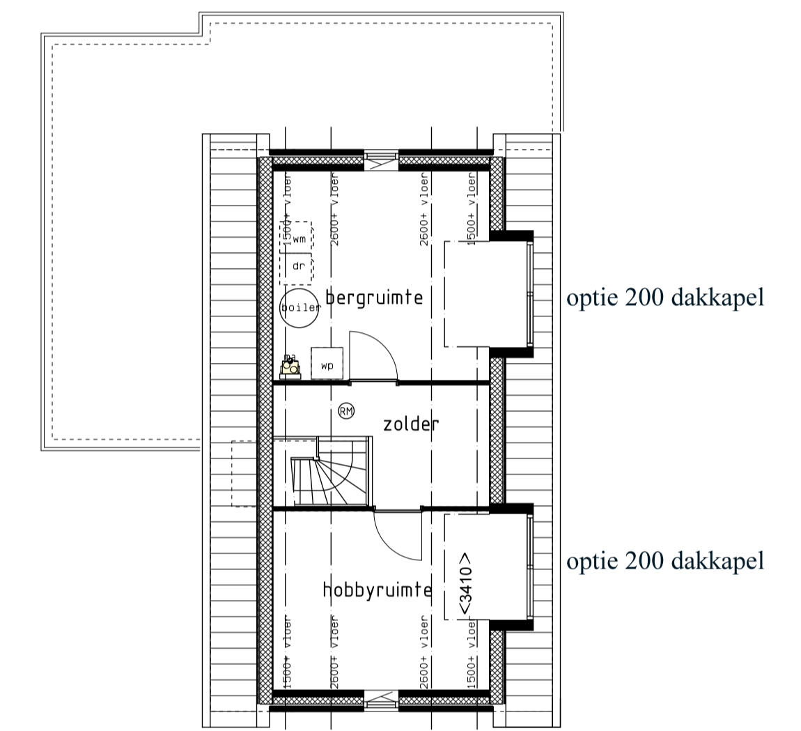
Zolder Verdieping
