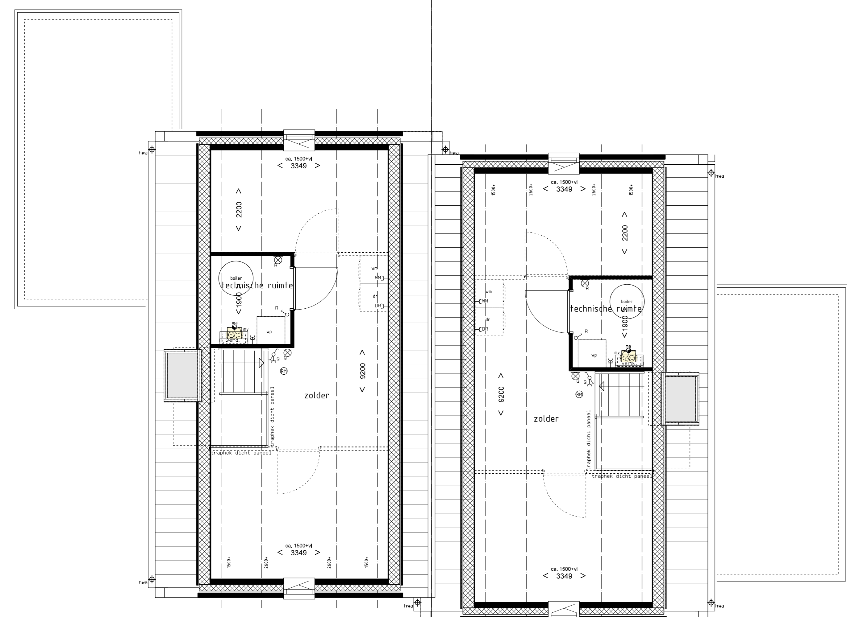
Zolder Verdieping
